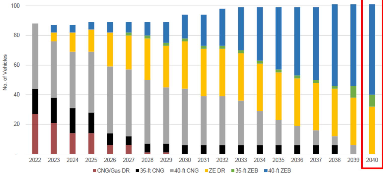
GCTD fleet composition through 2040 by vehicle type and technology
