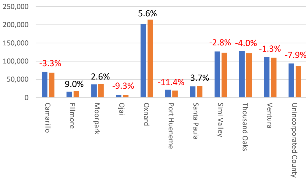
Population: 2016 to 2050
